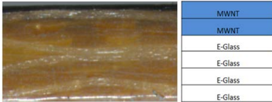
Figure 5. The image on the left is an optical microscope photo taken at 22 \times magnification. The image shows the MWNT plies (top black), 4 layers of woven E-glass (light yellow), and the epoxy resin, BMI, used in making the composite. On the right is a schematic of the nanocomposite being studied. There are two plies of MWNTs on a substrate made of 4 plies of E-glass, with the resin layer being included in with the E-glass.
