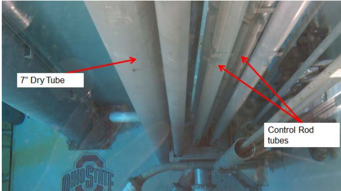
Figure 13. The OSURR as viewed from above looking into the cooling pool at the reactor. The dry tube is marked on the left and the reactor control rod tubes are also marked. The reactor is at the bottom of the pool.
